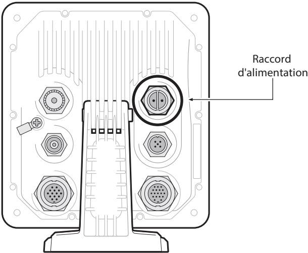
Figure 15 Raccord d'alimentation
