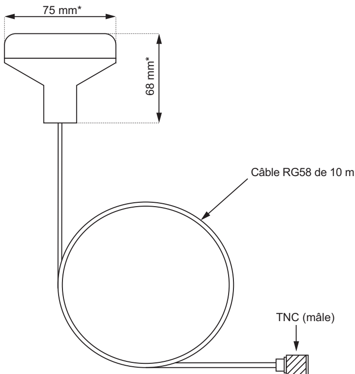
Figure 31 Antenne GNSS
