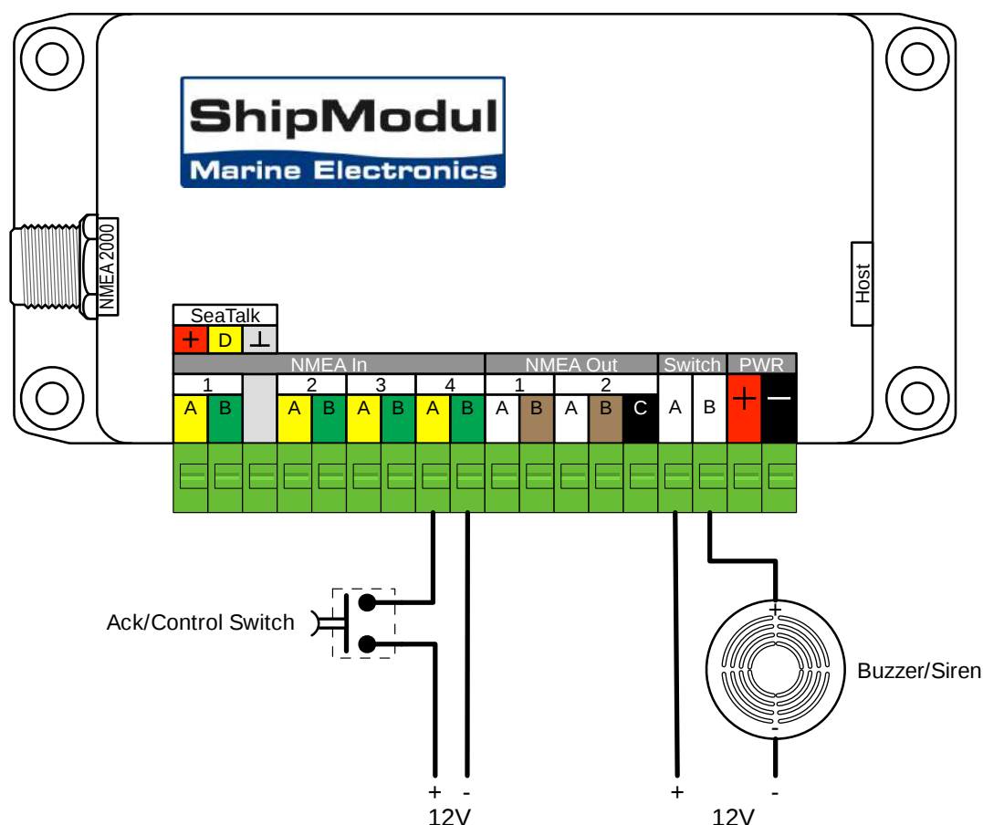
Figure 62: Connexions AIS MOB Alarm
